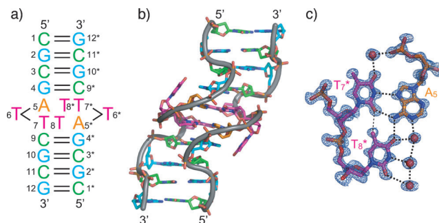
Figure 3. a) Secondary structure and b) crystal structure of the non-helical DNA duplex obtained in the absence of Hg II , and c) local 2|F_o| - |F_c| map for an A 5 -T 7 *-T 8 * triplet in the DNA duplex contoured at 1\sigma level. Hydrogen bonds and a C-H...O interaction are represented by thick and thin dashed lines, respectively. Oxygen atoms of water molecules are shown as red spheres.
